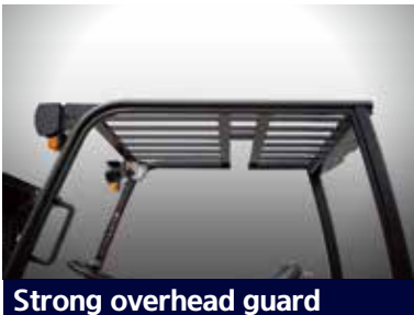
Strong overhead guard Exceeding the EEC and ANSI regulations, the overhead guard offers great protection combined with excellent all around visibility.
